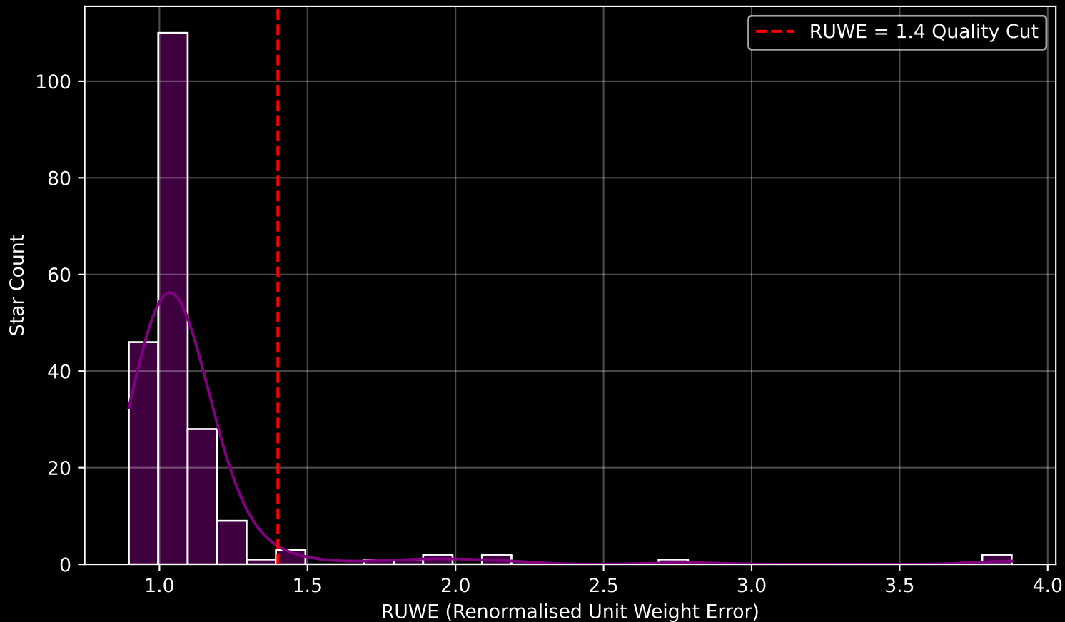
GAPOGEE DR17 Field [109-12] RUWE Distribution (n= 206)
