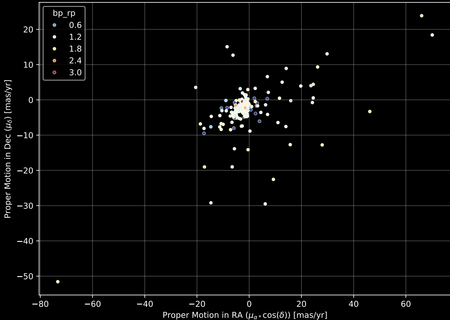
APOGEE DR17 Field: [109-12] Proper Motion Diagram (n= 212)
