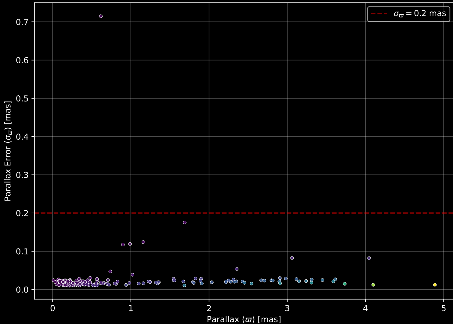
APOGEE DR17 Field: [109-12] Parallax Quality (n= 212)
