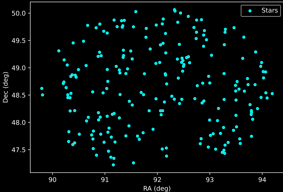
APOGEE DR17 Field: [109-12] Proper Motion Vectors for Gaia Star Field (n= 212)
