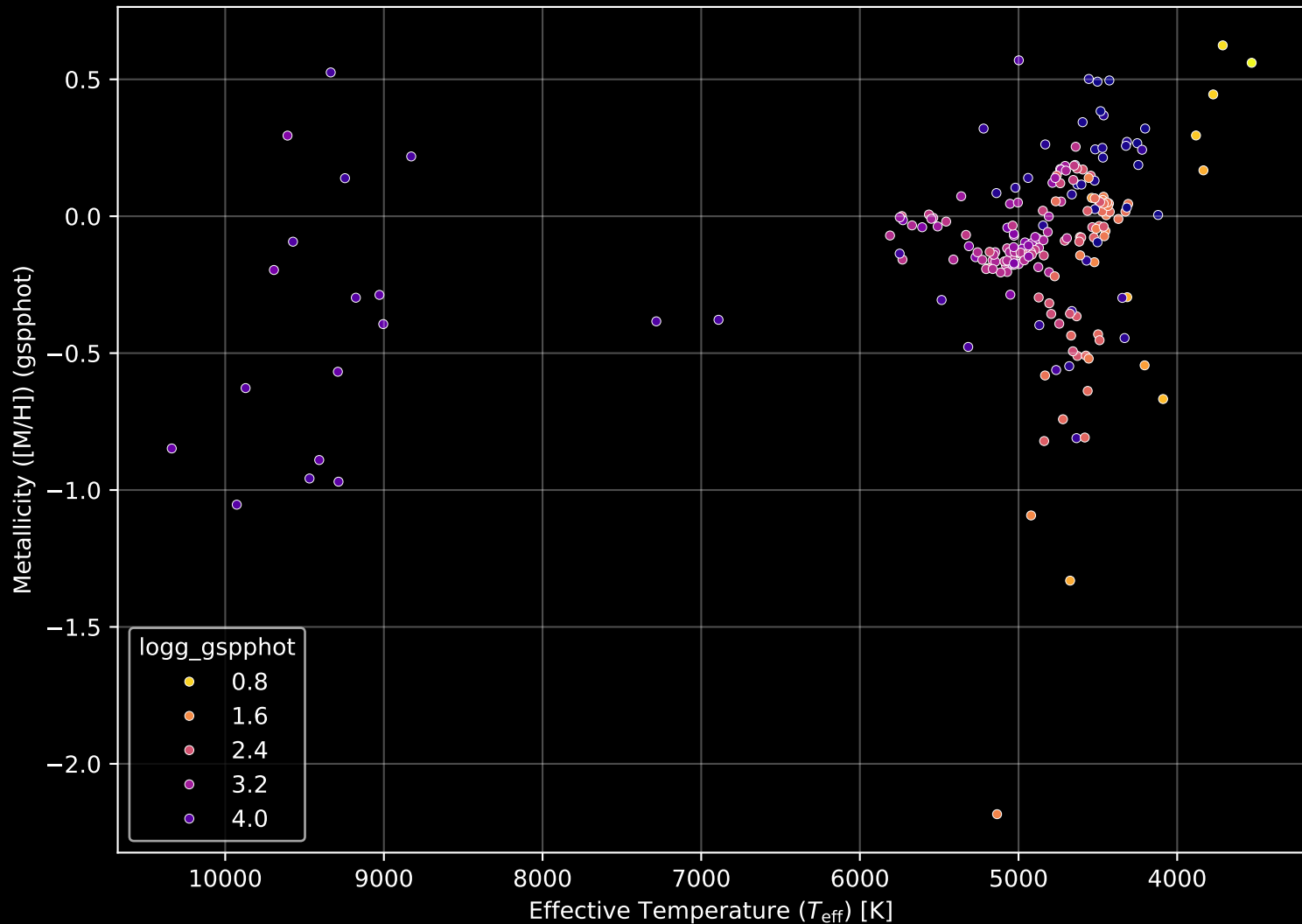
APOGEE DR17 Field: [109-12] Stellar Population Parameters (n= 212)
