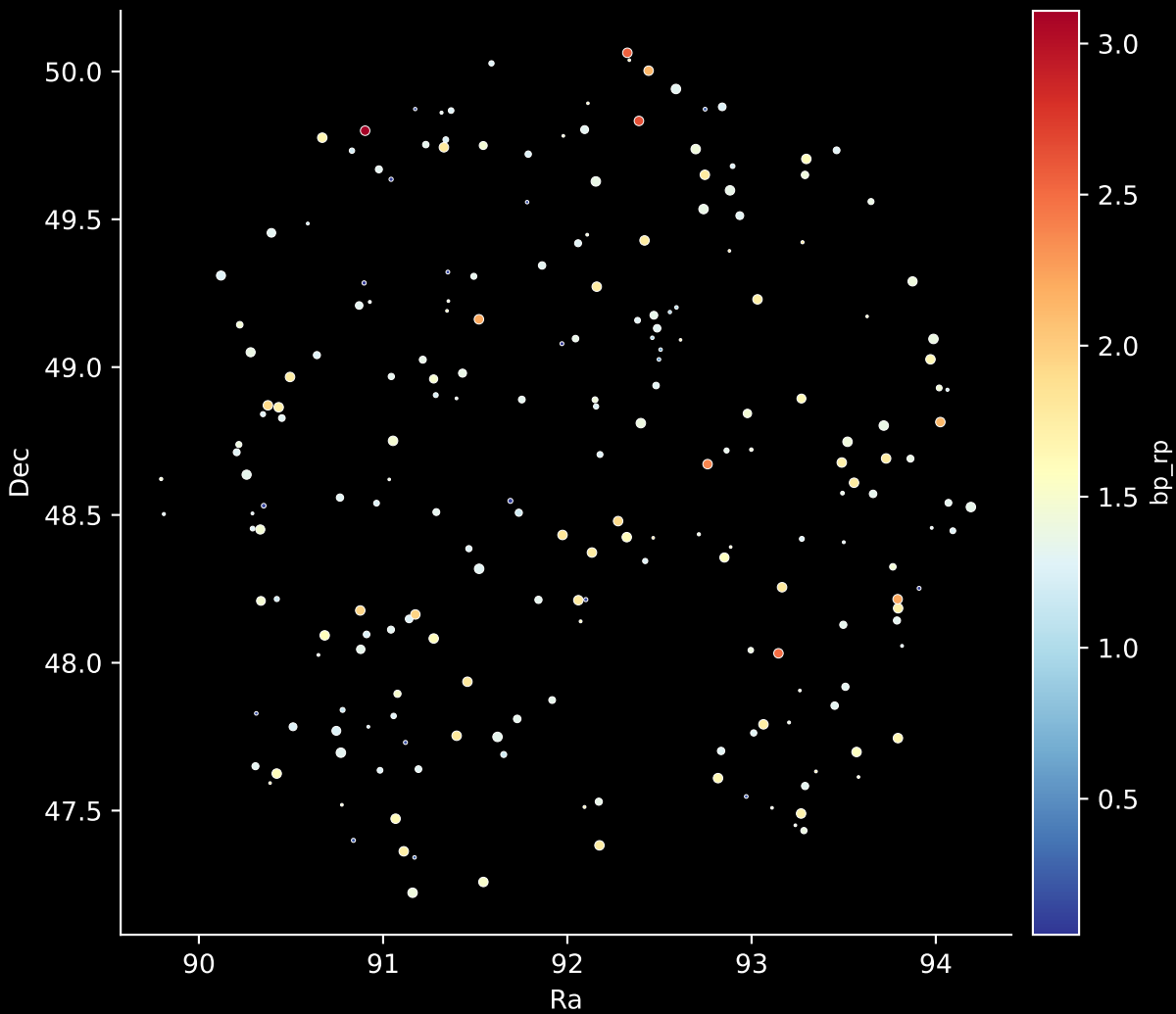
APOGEE DR17 Field: [109-12] Stars: 212
