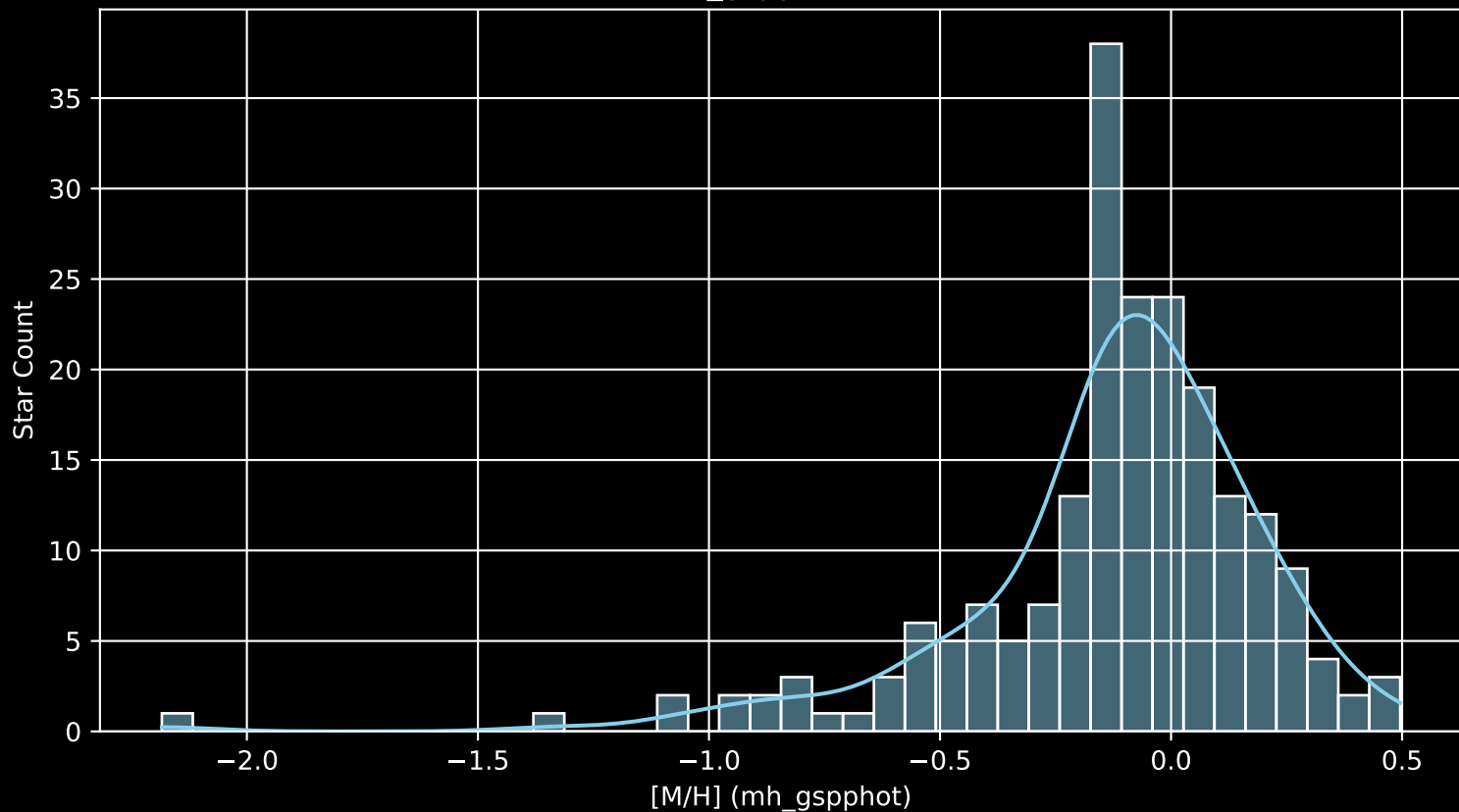
APOGEE DR17 Field: [109-12 [M/H] (mh_gspphot) (n= 207)
